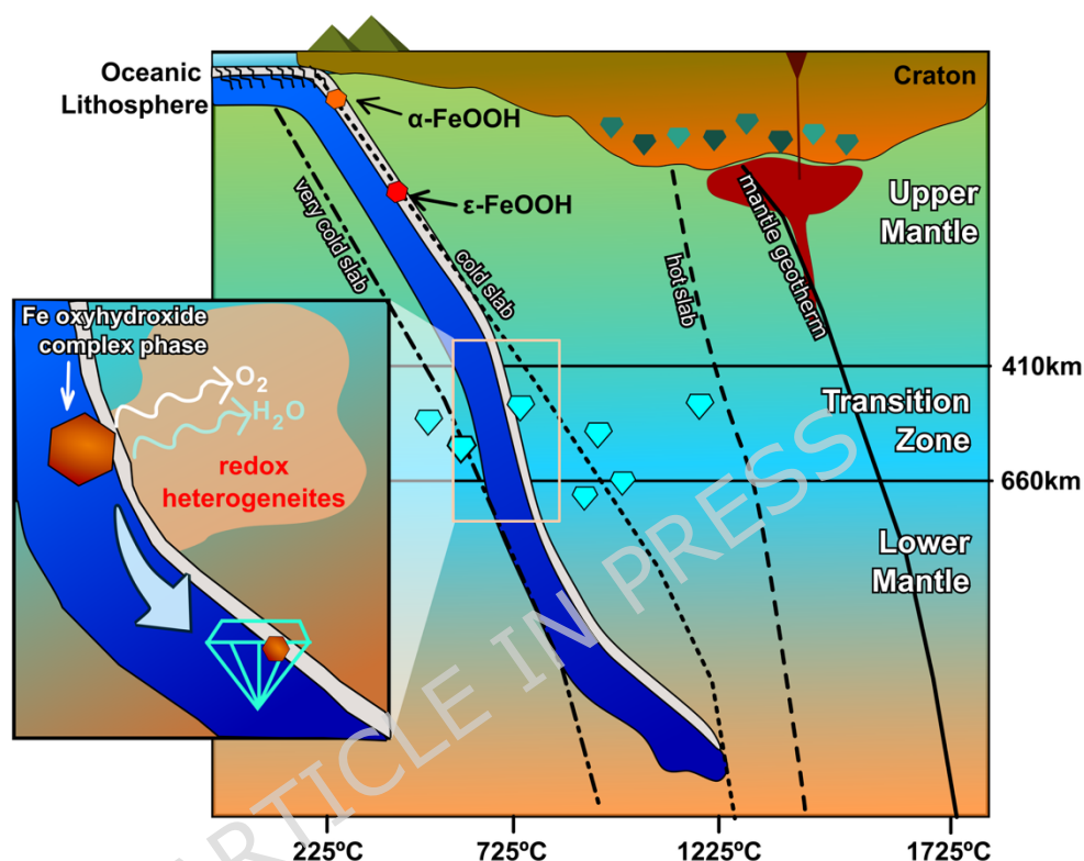
Figure 5. Schematic cross-section showing a cold subducted slab descending through the mantle transition zone into the deep mantle. The cold, very cold slab and hot geotherms are represented by dashed lines (Refs. 54,55). The mantle geotherm is represented by the black line (Ref. 57). The \alpha\text{-FeOOH} found in the oceanic crust or lithosphere transforms into its high-pressure polymorph, \epsilon\text{-FeOOH} at \sim 230 km depth ( \sim 7 GPa) (Refs. 26,39). As the slab descends to deeper regions, the \epsilon\text{-FeOOH} begins to break down into \text{Fe}_2\text{O}_3 and \text{Fe}_3\text{O}_4 , releasing volatiles into the surrounding rocks (inset figure). This transformation may form localized redox heterogeneities in the mantle. The phase transformation is incomplete, forming a heterogeneous Fe oxyhydroxide assemblage in the crystal (inset), which is then trapped in a diamond, potentially crystallized from fluids and melts released by the slab (inset figure) (Refs. 3,56).
