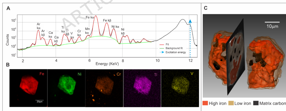
Figure 2. Nano-X-ray Fluorescence (n-XRF). (A) n-XRF spectrum with the identified main element emission lines. Elements such as Ar, Ca, and Mn are from the surroundings and do not belong to the studied mineral; (B) 2D n-XRF map formed by the integrated spectra corresponding to the different elements Fe, Ni, Cr, Ti, and V; (C) nano-tomography with fluorescence contrast (n-XFCT), segmented in three levels, emphasizing higher and lower amounts of Fe and the channels filled with diamond or carbon matrix.
